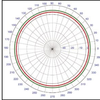
Radiation Patterns H - Plane @ 850 MHz 5.12 dBi H - Plane @ 1920 MHz 6.12 dBi
