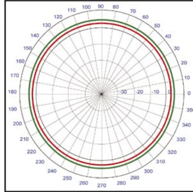
Radiation Patterns H - Plane @ 850 MHz 4.5 dBi H - Plane @ 1920 MHz 5.9 dBi
