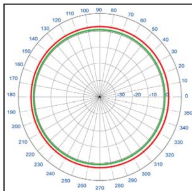
Radiation Patterns H - Plane @ 920 MHz H - Plane @ 1795 MHz
